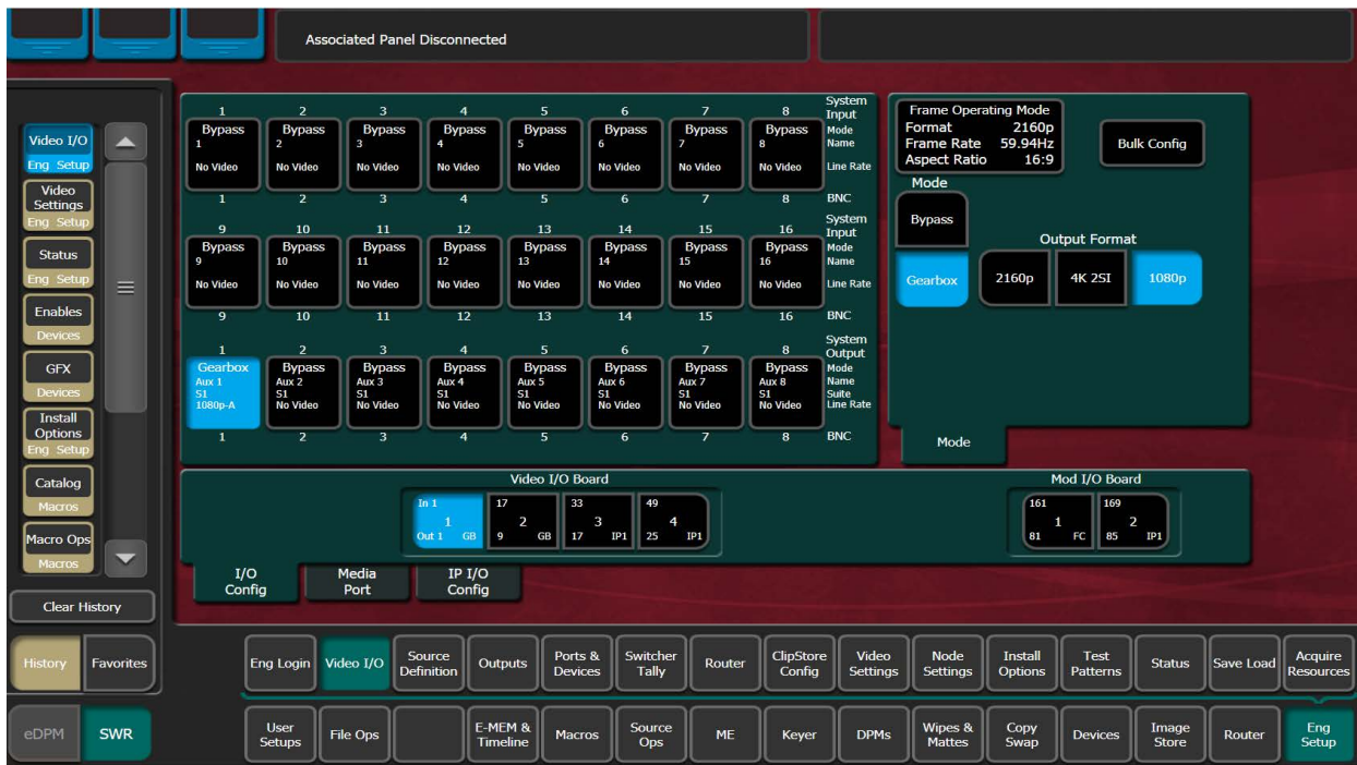
16 x 8 SDI GearBox IO Board – Output Mode set to GearBox, Output Format set to 1080p
